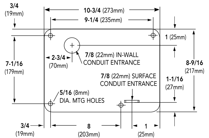
Figure 3 - A-T Series Surface Mount
