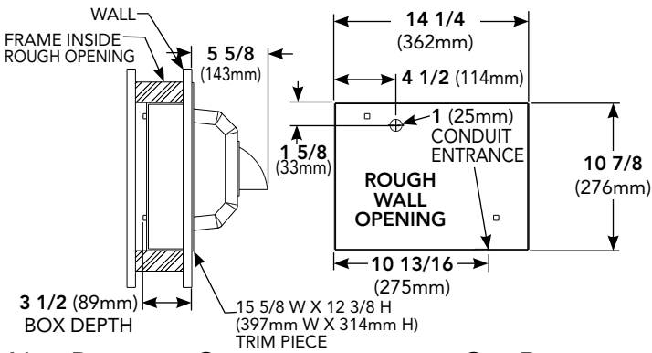
Figure 2 - DR-R Series Recessed Mount
