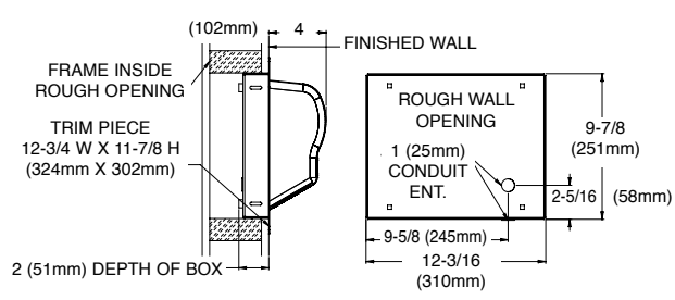
Figure 2 - EXT-MR Series Recessed Mount
